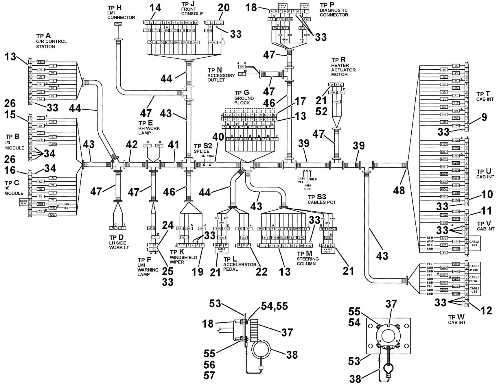
DETAIL DIAGNOSTIC CONNECTOR J1939 DIAGNOSTIC CONNECTOR ASSY
